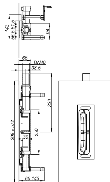
drain body DallFlex Plan
